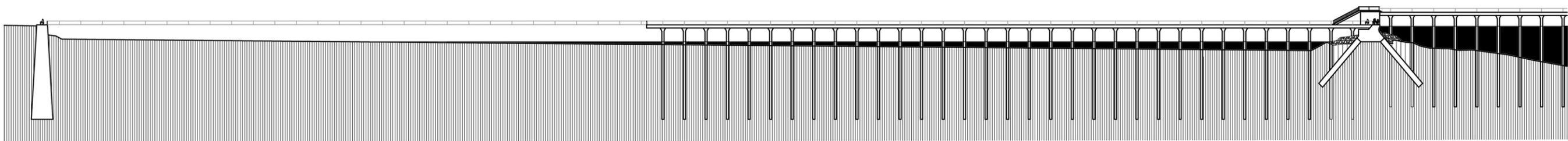
brittlebank park: section through seawall, retention park, boardwalk
